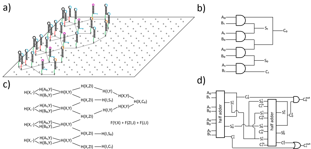
Figure 12: Multiple representations ((a) through (c)) of a half-adder circuit on an origami tile. As shown in (d), another half-adder and simple logic can be added to make a full adder.
